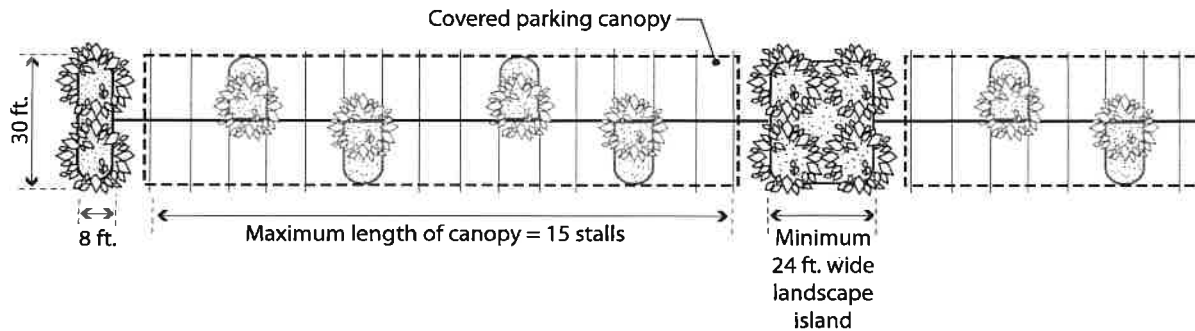
Figure 18.90.050.B.6. Adjacent Canopies
