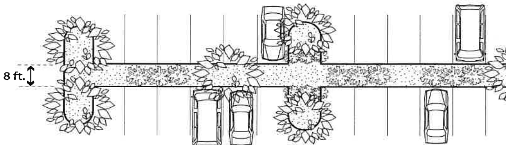
Figure 18.90.050.C.2. Double-Row Parking
