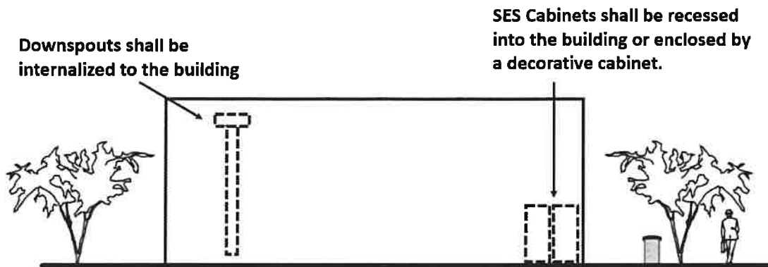
Figure 18.80.110.A.3. Screening of Exterior Wall-Mounted Equipment
