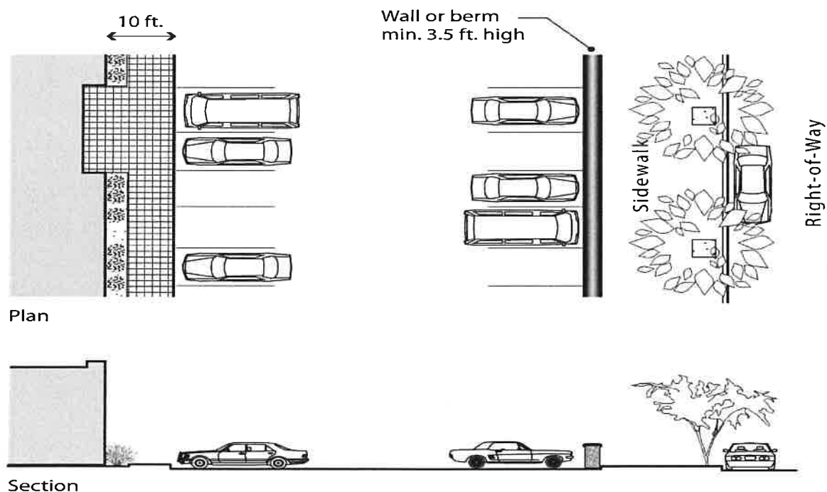
Figure 18.80.110.H. Screening and Separation of Parking Areas
