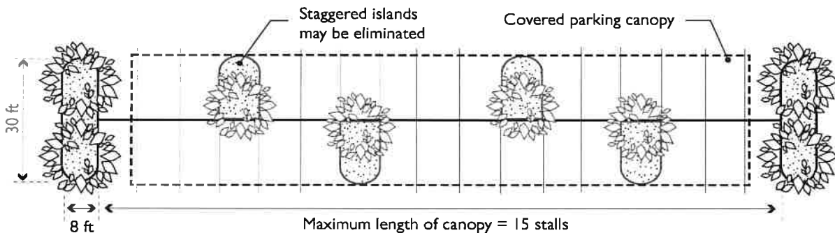
Figure 18.90.050.B.7. Covered Canopies
